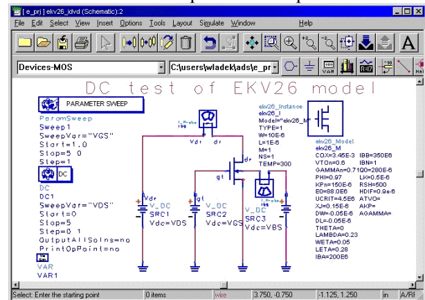
Fig. 7. ADS schematic view of a simple circuit with the EKV model implemented using ADMS tool.
