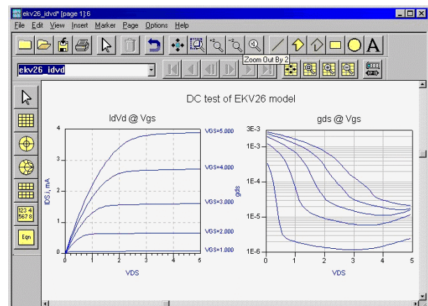
Fig. 8. Results of output current and conductances simulations.
