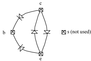
Fig. 1. Branch assignment in the HBT model.
